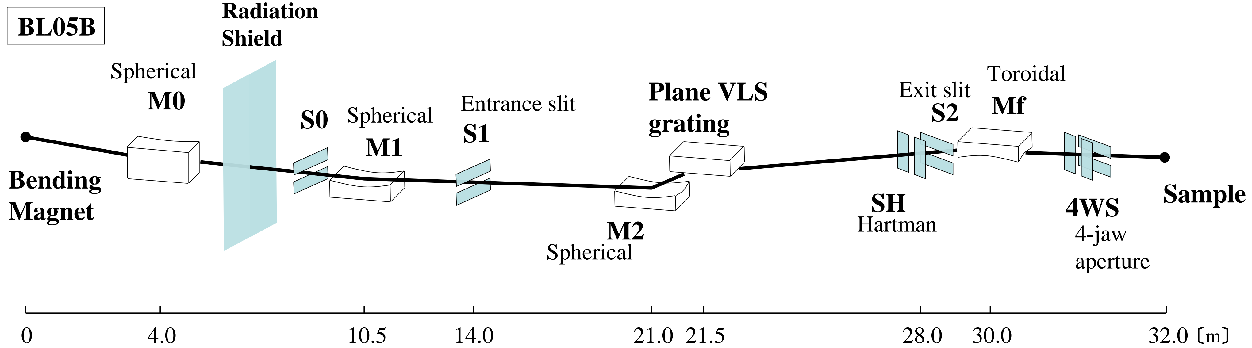
Layout of BL05B
